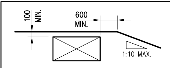
TYPICAL TENDON DETAIL AT PENETRATIONS & OPENINGS
