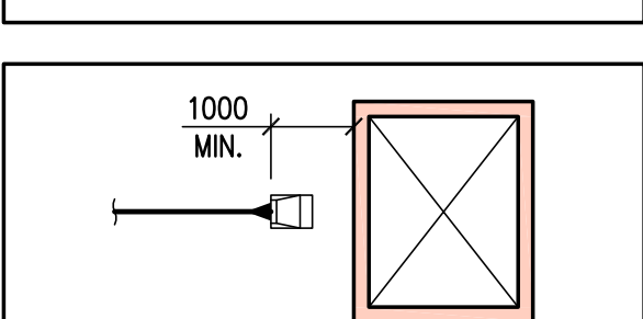
TYPICAL MIN. STRESSING DISTANCE FOR PAN TO WALL
