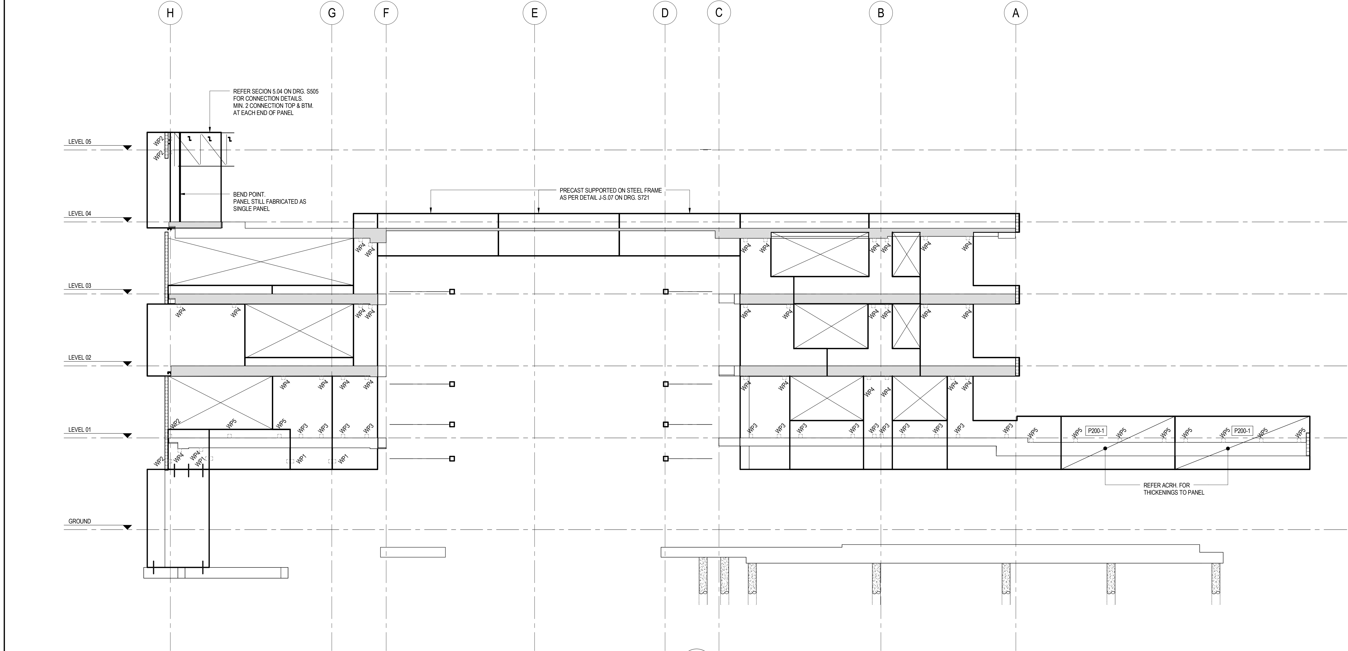
ELEVATION E.23 SCALE 1:100 NOTE: ALL PANELS P180-1 UNLESS NOTED OTHERWISE.
