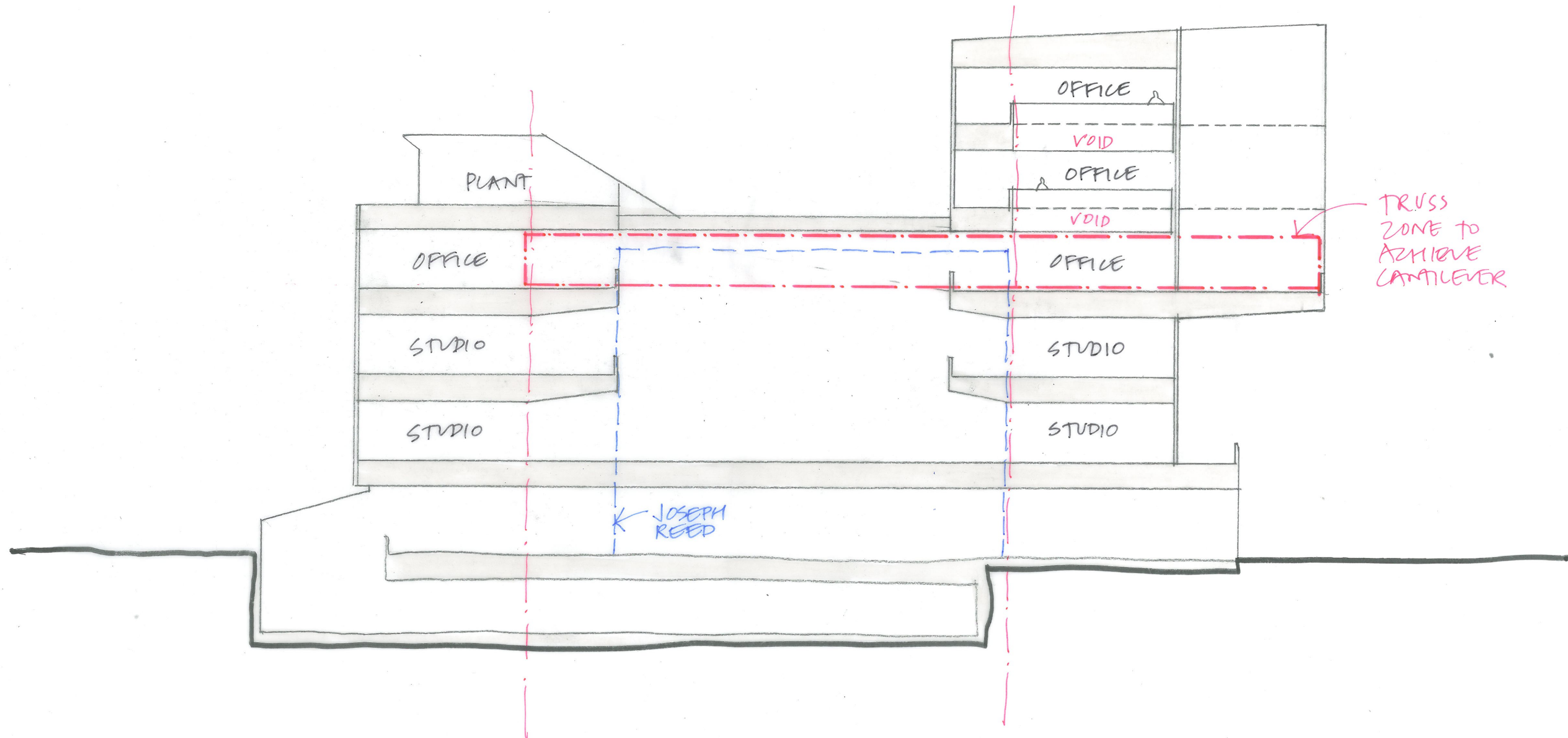
CROSS SECTION 1/200 EASTERN FAB LAB
