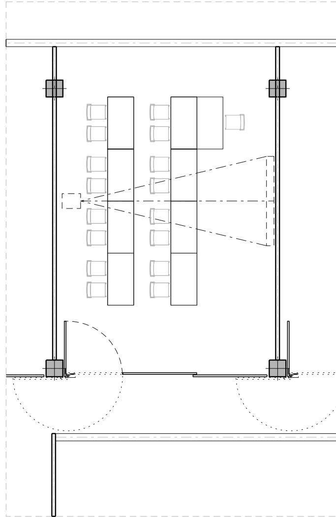
Option A - Pivoting / Sliding Entry Door
