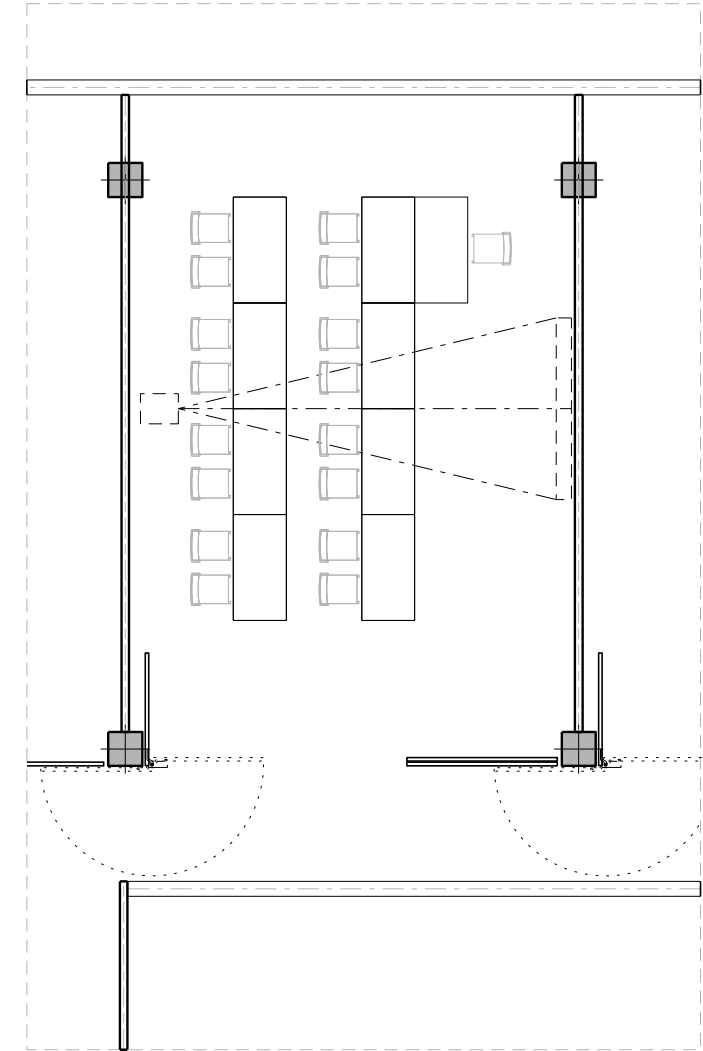
Option A - Pivoting / Sliding Half Open Entry
