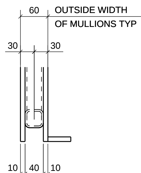
DETAIL 1
