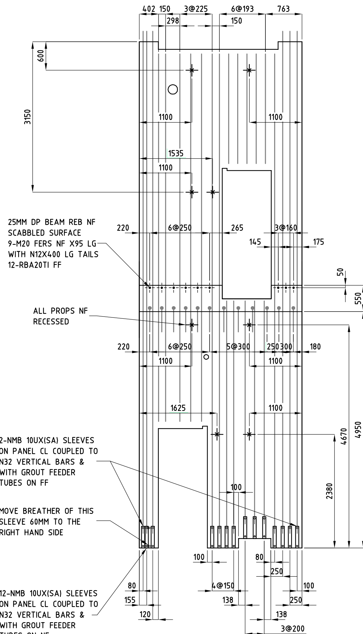
BTM SLEEVE LAYOUT & NF REBATE DETAILS
