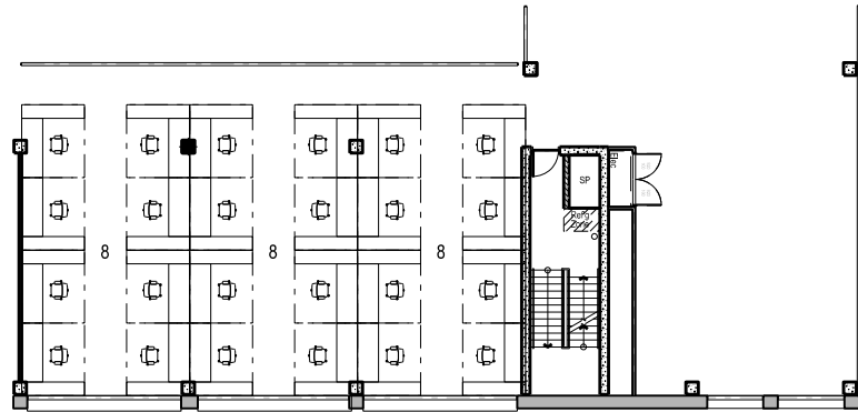
6m 2 + circulation = 24 RHDS workspaces
