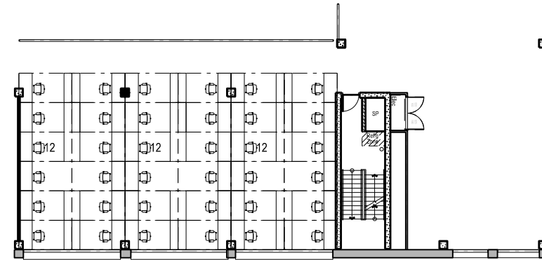
5m 2 incl circulation = 36 RHDS workspaces
