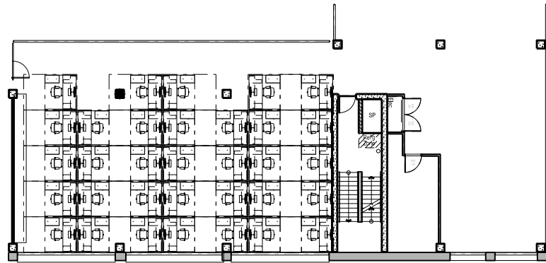
Schematic Design Layout 4.85m 2 including circulation = 33 RHDS workspaces
