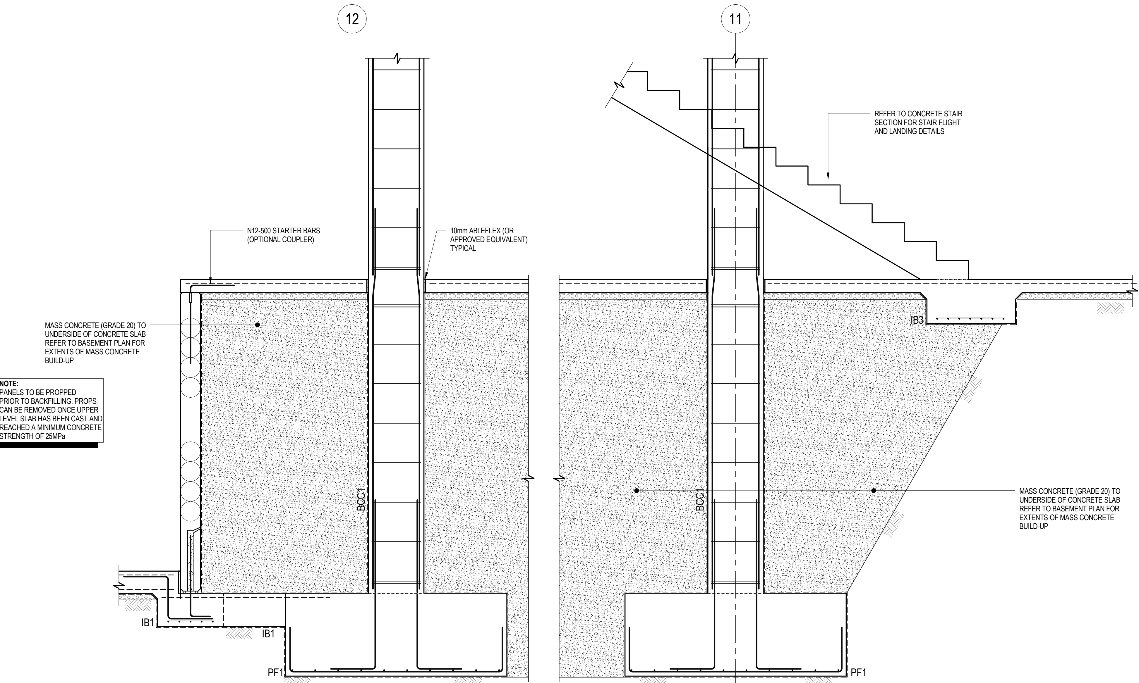
SECTION B.04 SCALE 1:20 S011
