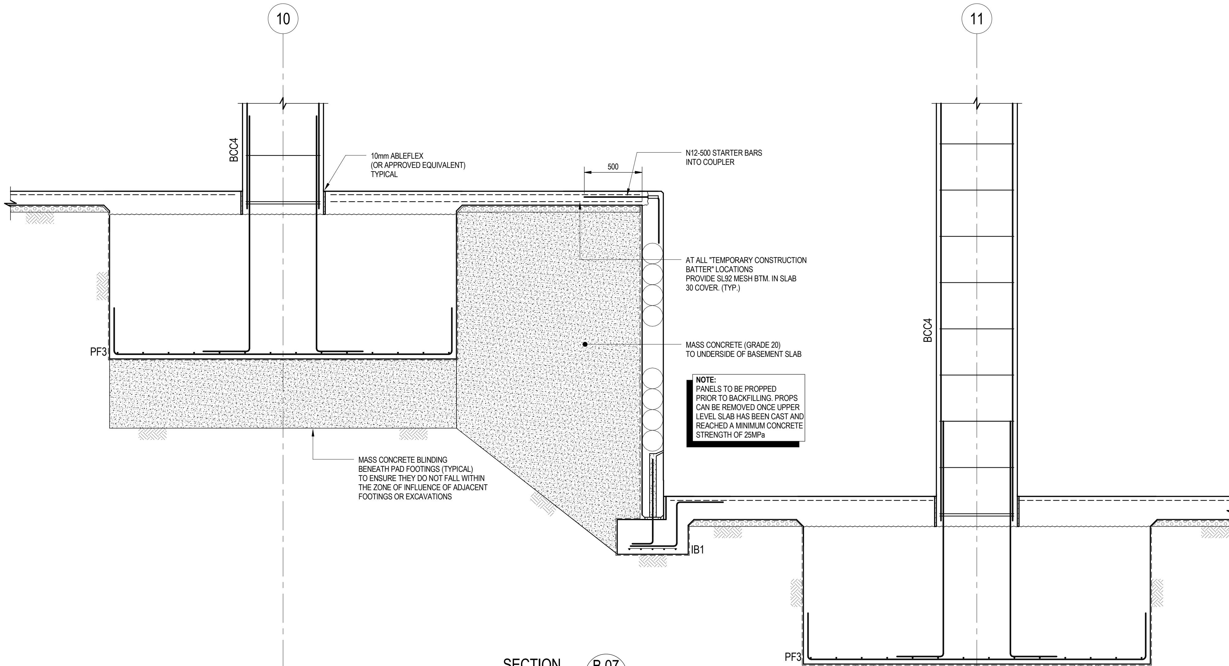
SECTION B.07 SCALE 1:20 S011
