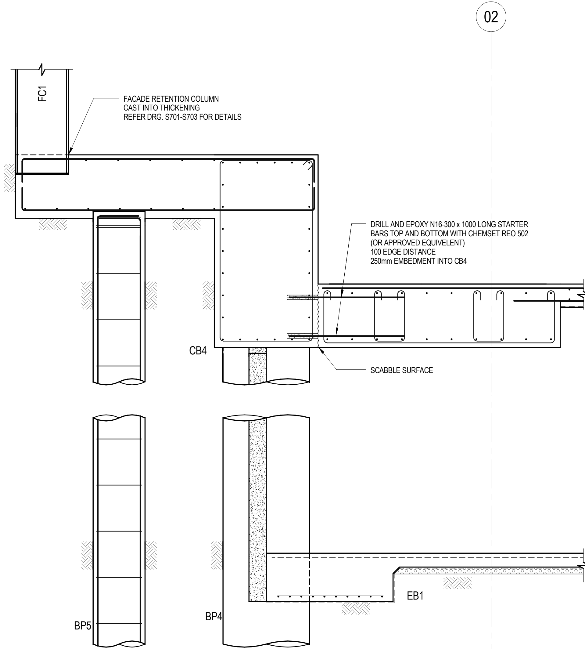
SECTION B.05 SCALE 1:20 S011
