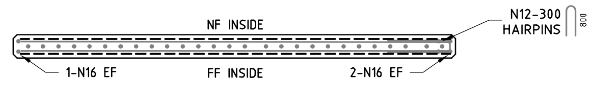
SECTION B-B
