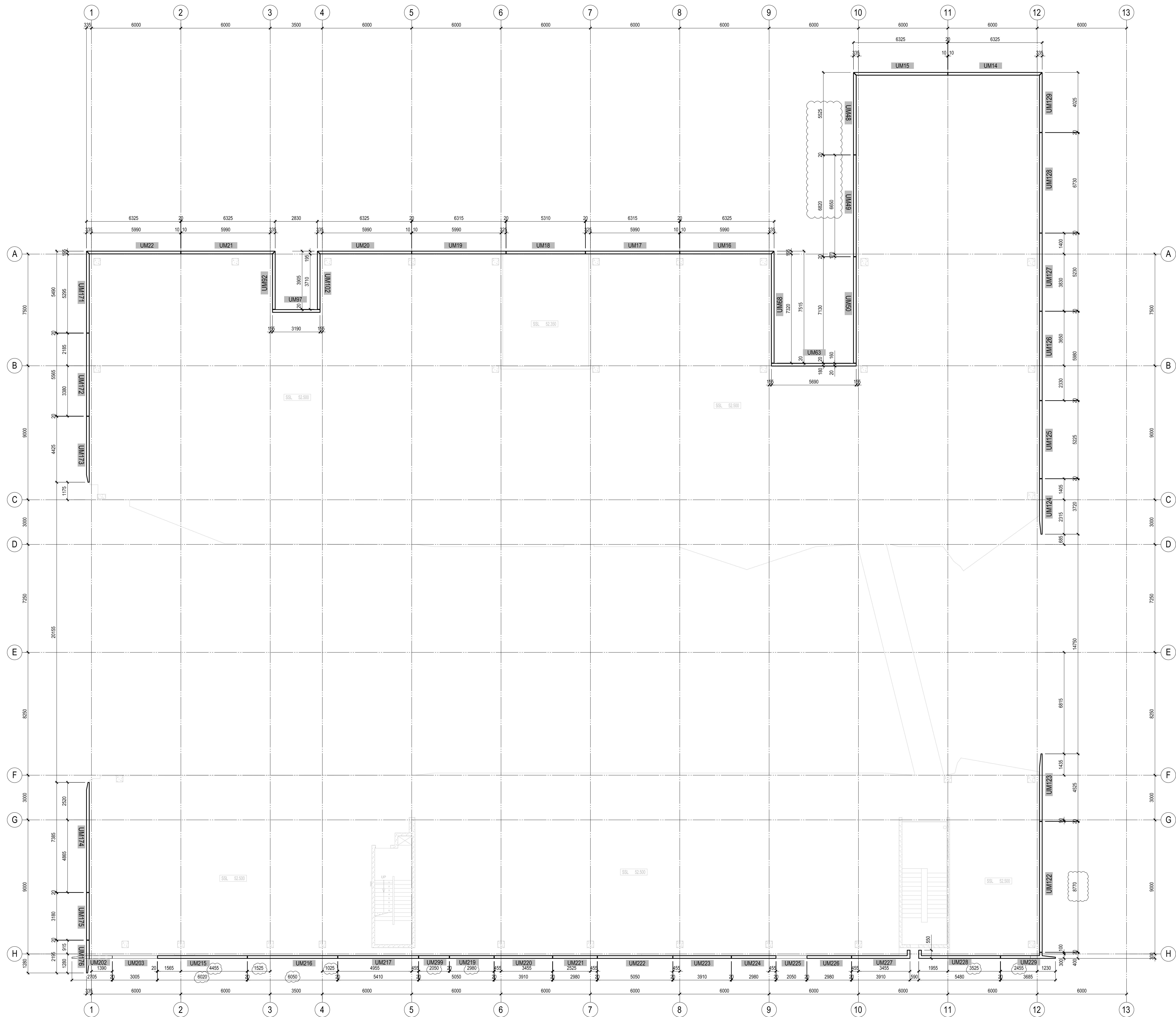
PRECAST PANEL PLAN LAYOUT LEVEL 2
